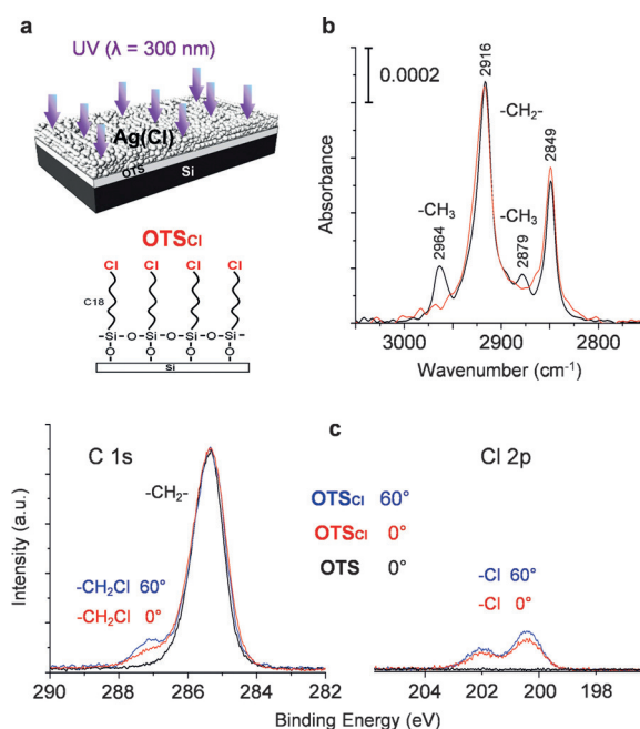
Figure 2. Interfacial solid-phase chlorination of OTS/Si monolayer using a thin Ag(Cl) film as reagent (see text): a) Reaction set-up and the molecular structure of the reacted monolayer, \text{OTS}_{\text{Cl}}/\text{Si} (representation as in Scheme 1). b) FTIR spectra (as in Figure 1b) of a pristine OTS/Si monolayer (black trace) and same monolayer after 30 min UV irradiation through a ca. 50 nm-thick Ag(Cl) film and its subsequent dissolution ( \text{OTS}_{\text{Cl}}/\text{Si} , red trace). c) XPS spectra of a pristine OTS/Si monolayer (black trace, 0^\circ emission angle) and the \text{OTS}_{\text{Cl}}/\text{Si} monolayer at 0^\circ (red trace) and 60^\circ (blue trace) emission angles. To facilitate a direct comparison of the relative angle-dependent intensities of the Cl (Cl 2p) and \text{CH}_2\text{Cl} (C 1s) lines, all curves were normalized by adjusting the respective \text{CH}_2 (C 1s) peak intensities to the same arbitrary value.
